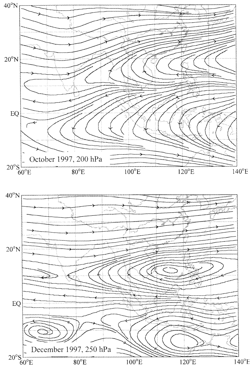
Figure 4. Monthly average streamlines at 200 hPa altitude in October and 250 hPa altitude in December 1997.
