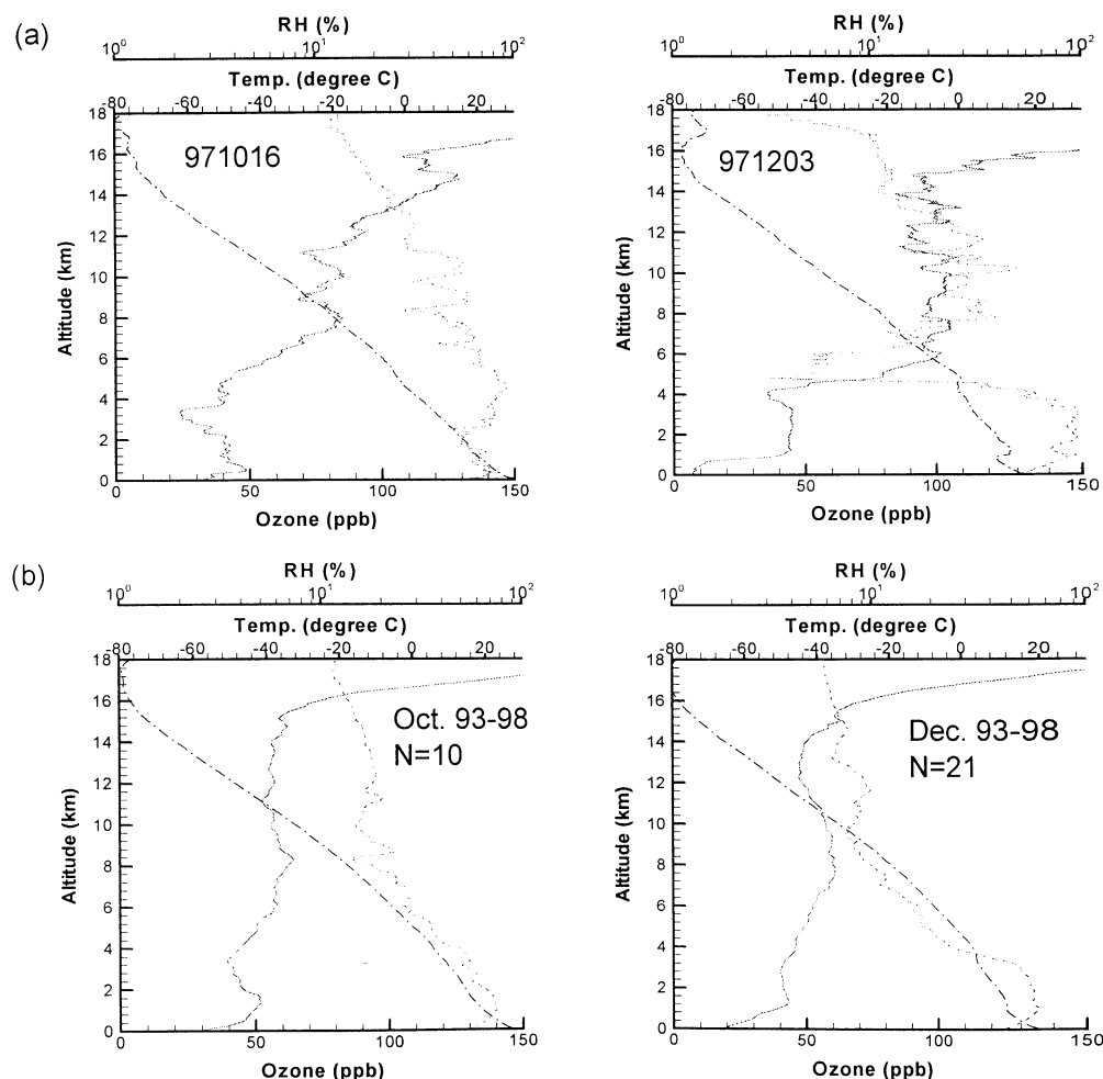
Figure 1. Ozone (solid), temperature (dot - dashed) and relative humidity (dashed) profiles on (a) October 16 and December 3, 1997, and (b) the monthly average ozone and relative humidity profiles in October and December from 1993 to 1998.
