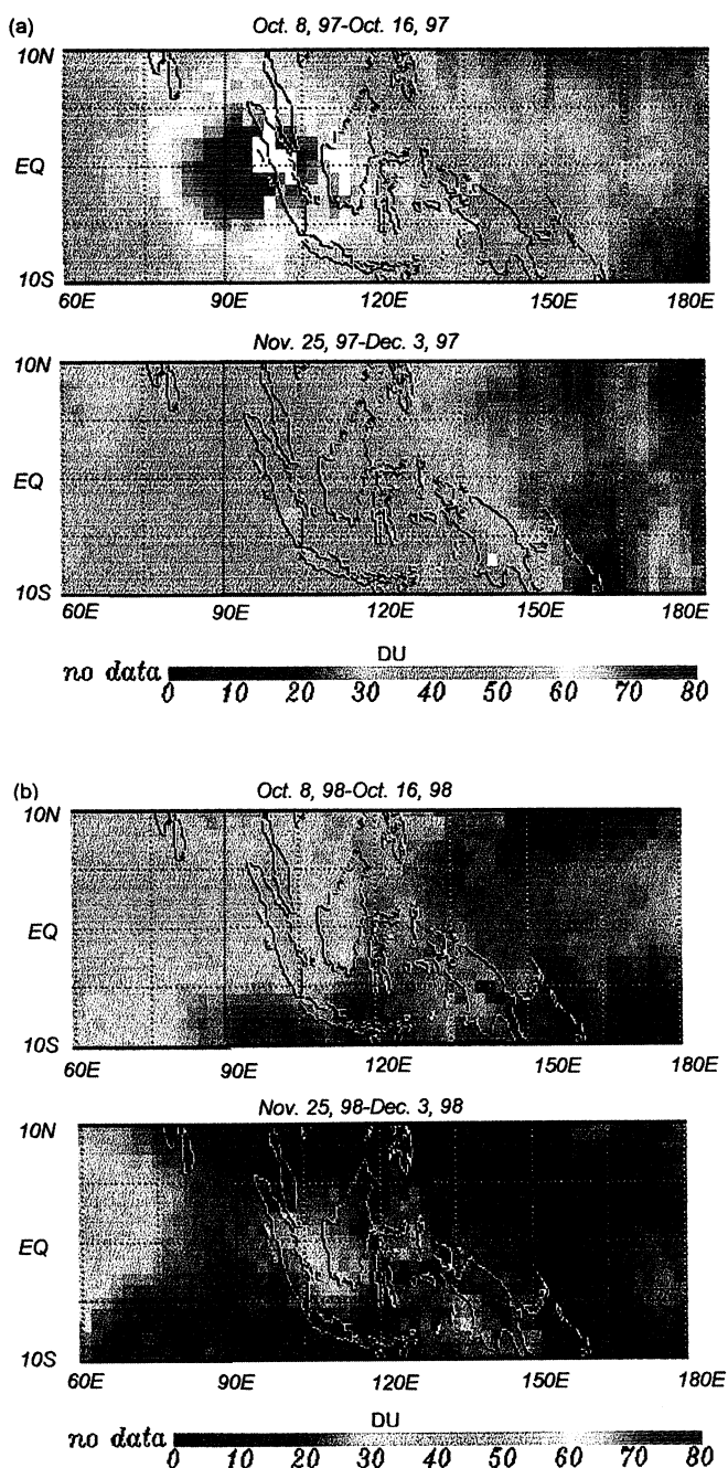
Plate 1. Tropical tropospheric ozone column from October 8 to 16 and November 25 to December 3 in (a) 1997 and (b) 1998. The enhancement is especially apparent over the Kalimantan and Sumatra regions as well as their immediate vicinities ( 10^{\circ}\text{S} , 75^{\circ}\text{E} – 10^{\circ}\text{N} , 120^{\circ}\text{E} ). The TOC ranged from 55 to 80 DU.
