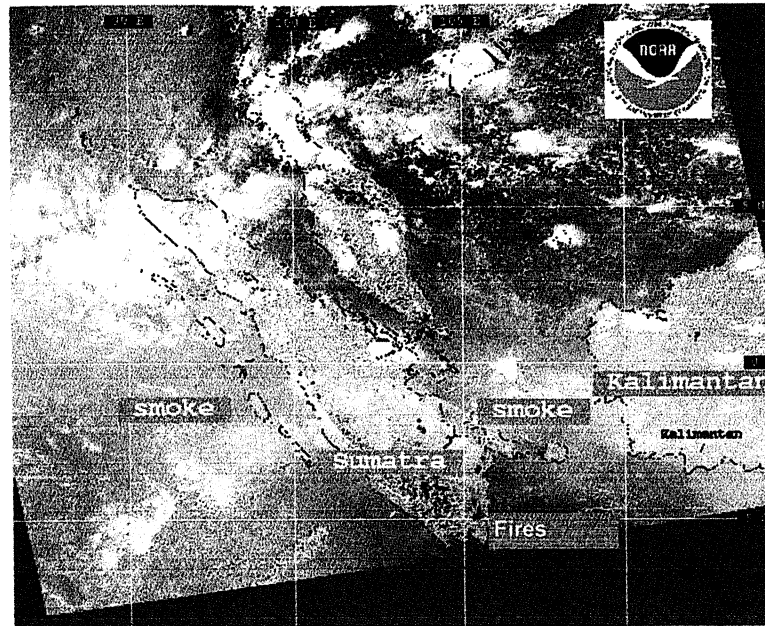
Plate 3. The AVHRR image on October 14, 1997. The locations of fires are red dots, and the smoke is a yellowish color. The cloud is white.
