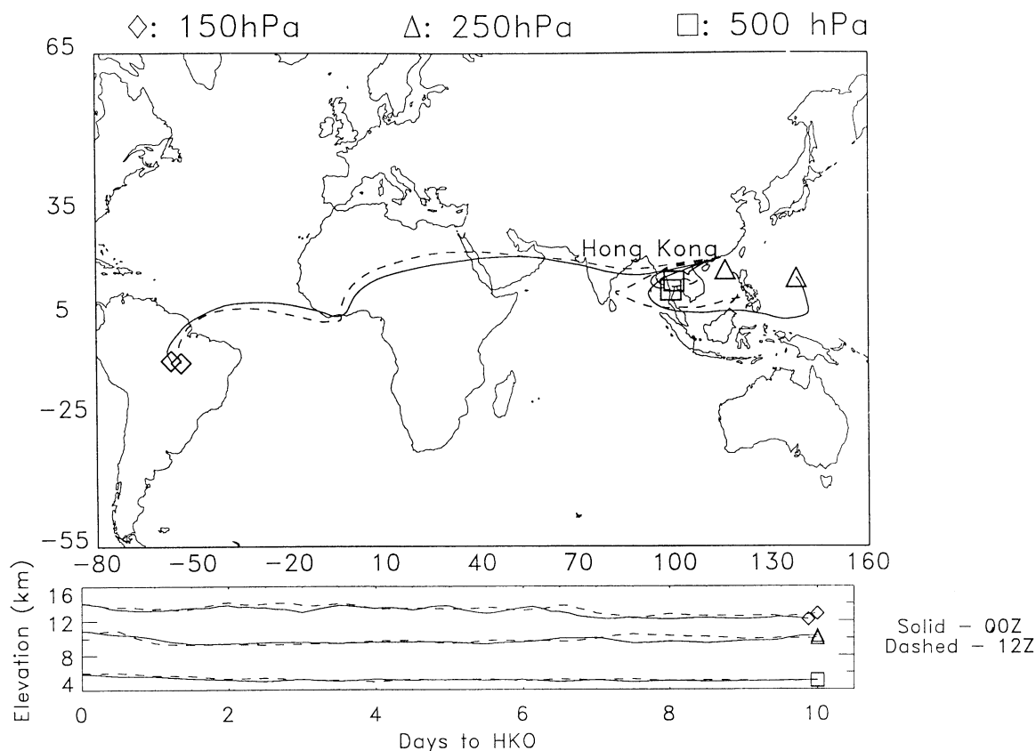
Figure 3. Back air trajectory on December 3, 1997 at 5.9 (500 hPa), 10.9 (250 hPa), and 14.1 km (150 hPa). Solid and dashed lines are for 00:00 and 12:00 UT, respectively.
