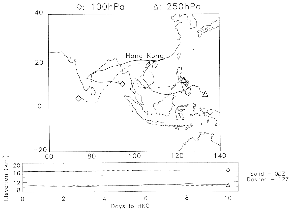
Figure 2. Back air trajectory on October 16, 1997 at 11.0 (250 hPa) and 16.6 km (100 hPa). Solid and dashed lines are for 00:00 and 12:00 UT, respectively.
