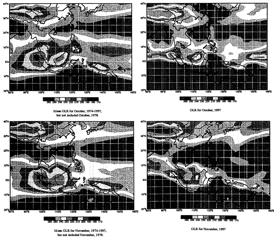
Plate 4. Monthly average OLR ( \text{Wm}^{-2} ) in the tropical and subtropical Western Pacific in October and November 1997 and from 1974 to 1997 (excluding 1978). High values of OLR correspond to suppressed convective activity.
