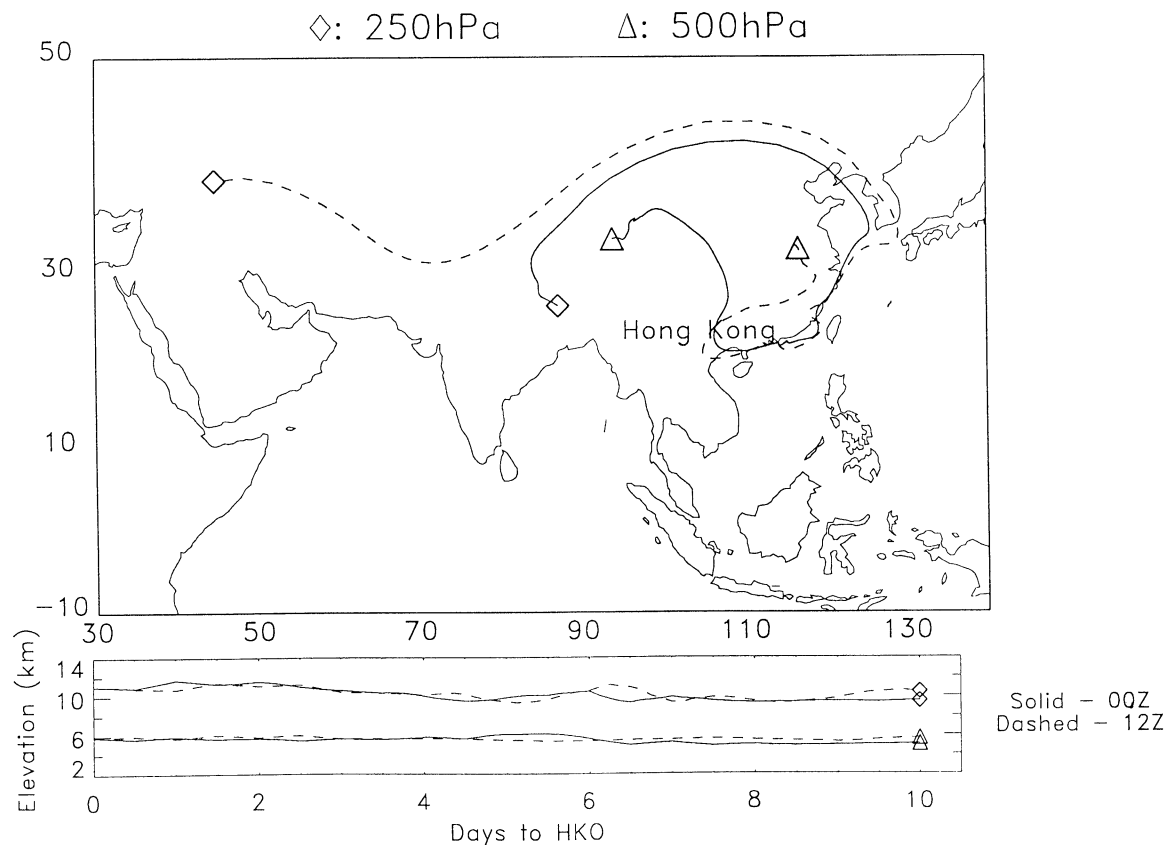
Figure 5b. Back air trajectory on August 13, 1997, at 5.9 (500 hPa) and 10.9 km (250 hPa). Solid and dashed lines are for 00:00 and 12:00 UT, respectively.
