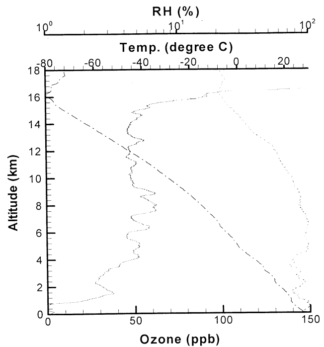
Figure 5a. Ozone (solid), temperature (dot - dashed) and relative humidity (dashed) profiles on August 13, 1997.
