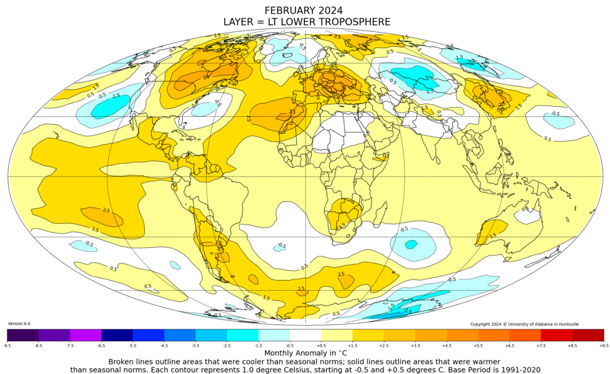
Figure. Lower tropospheric temperature anomalies for February 2024
