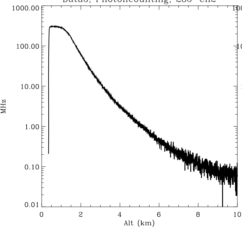
Data5, Photoncounting, 285-Ch2
