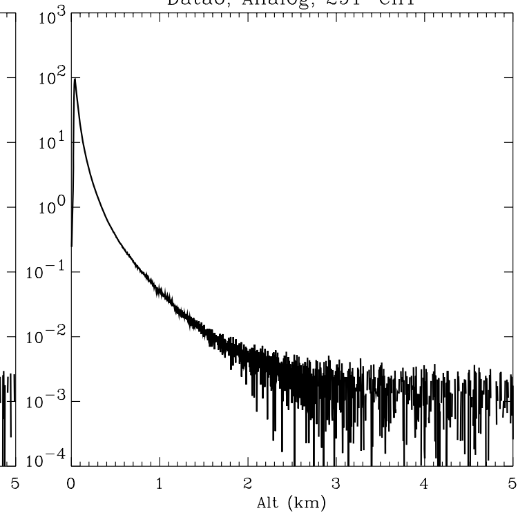
Data6, Analog, 291-Ch1
