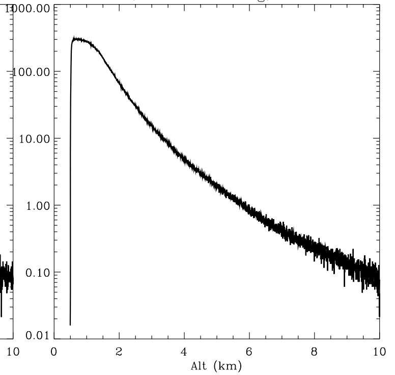
Data6, Photoncounting, 291-Ch2
