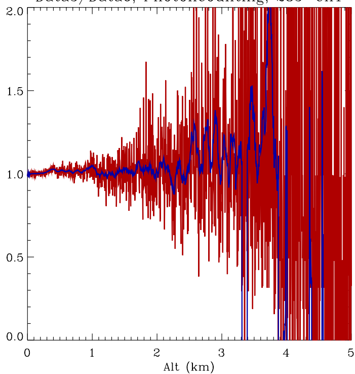
Data5/Data6, Photoncounting, 285-Ch1
