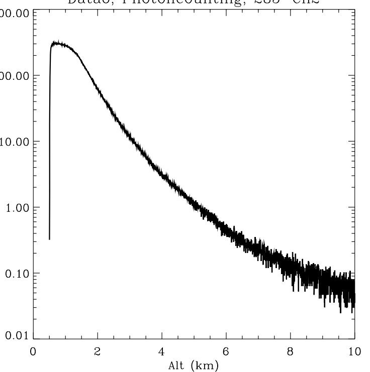
Data6, Photoncounting, 285-Ch2
